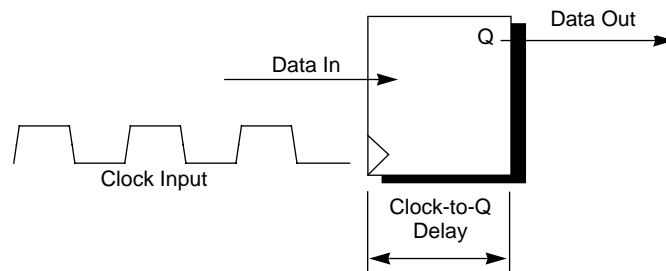
Figure 10-2 Clock-to-Q Delay
