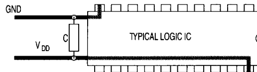
Figure 8. Decoupling Capacitor Placement
