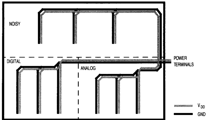
Figure 7. Single-Point Power System
