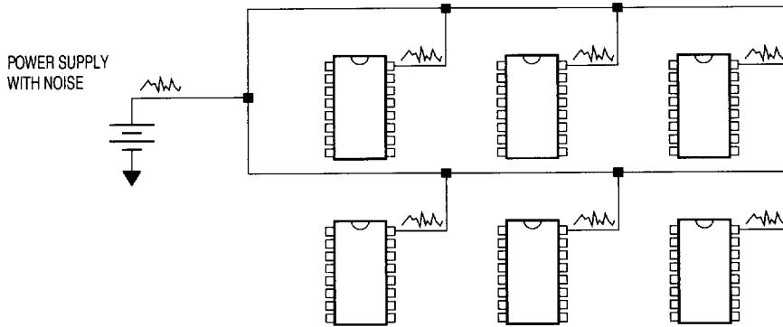
Figure 2. Conductor Coupled Noise
