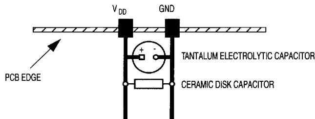
Figure 9. Power Terminal Decoupling Capacitor Placement
