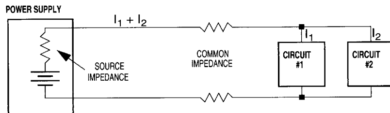
Figure 3. Coupling through Common Impedances
