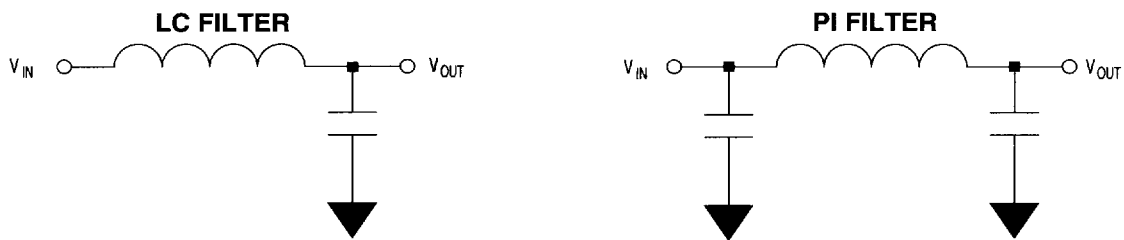
Figure 10. High Frequency Noise Filters
