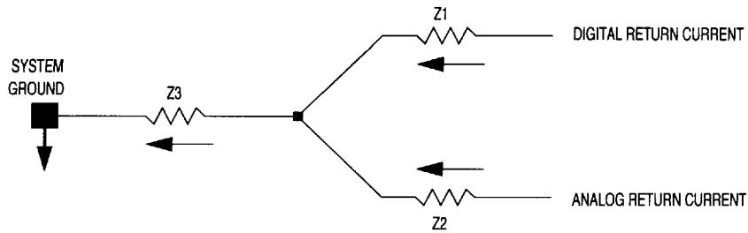
Figure 6. Common Impedance Coupling
