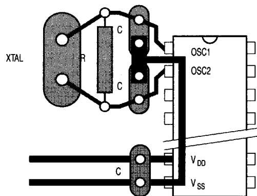
Figure 11. Crystal or Ceramic Resonator Circuit Layout
