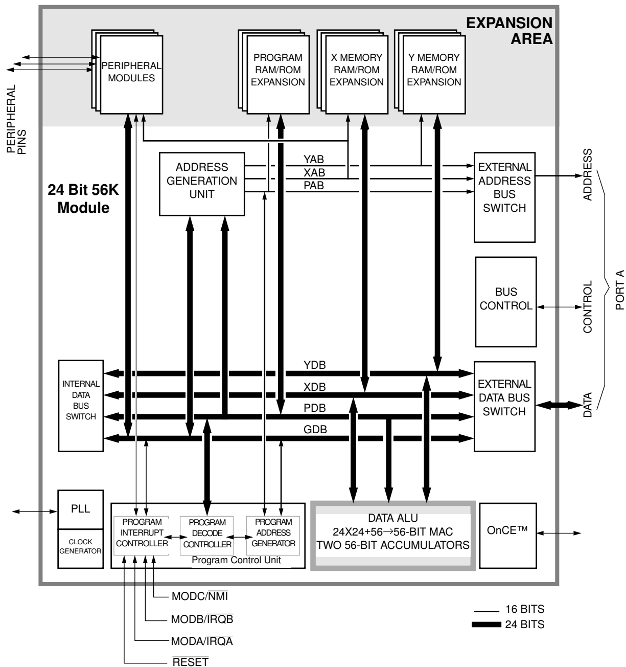
Figure 3-1 DSP56K Block Diagram
