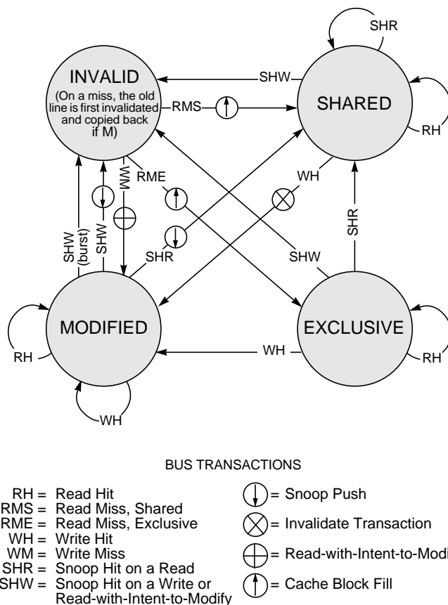
Figure 9-1. MESI Cache Coherency Protocol—State Diagram (WIM = 001)
