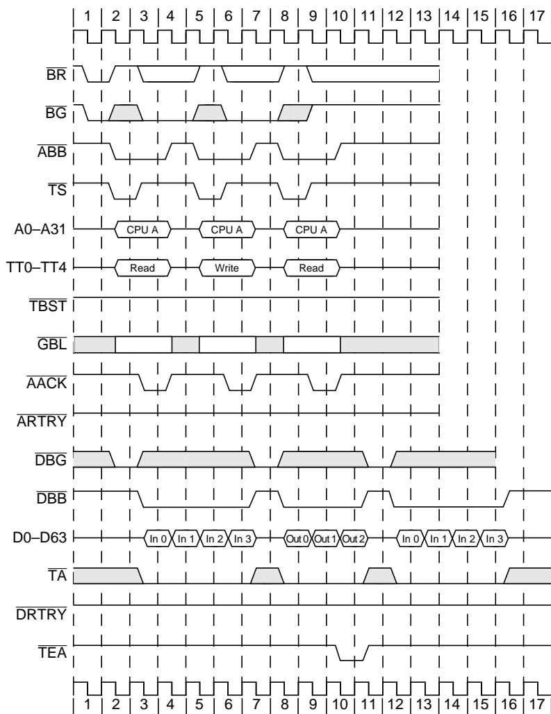
Figure 8-21. Use of Transfer Error Acknowledge (TEA)
