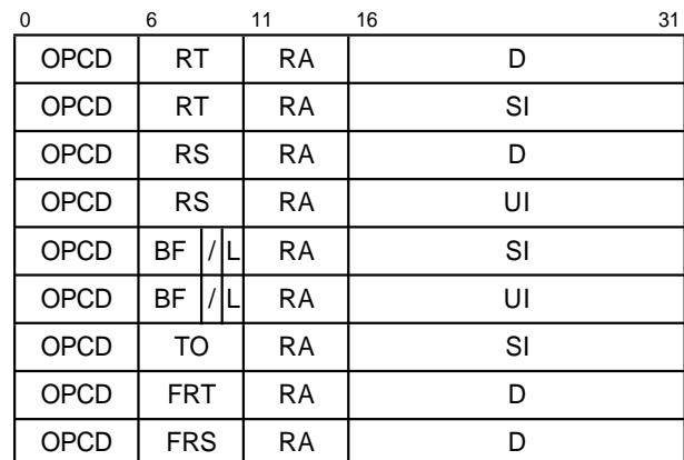
Figure 6. D instruction format
