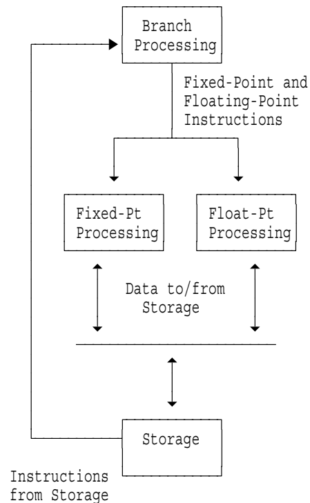
Figure 1. Logical processing model
