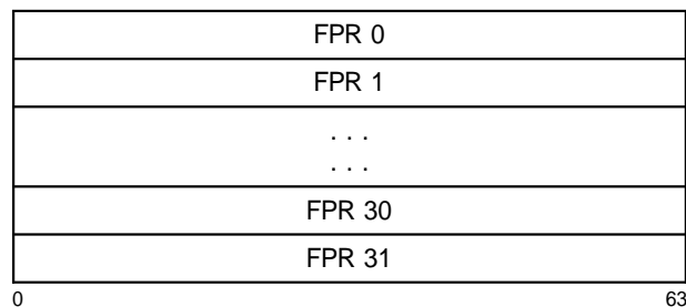
Figure 26. Floating-Point Registers
