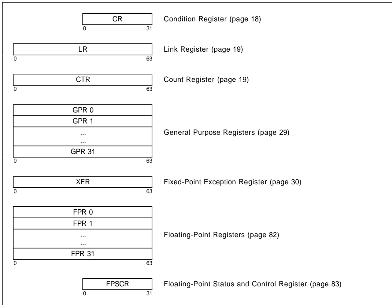
Figure 2. PowerPC user register set
