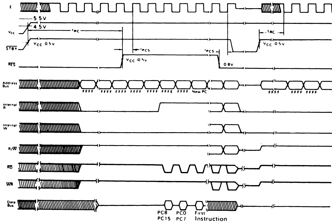
Figure 11 Reset Timing
