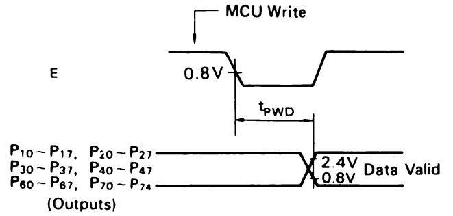
Figure 6 Port Data Delay Times (MCU Write)
