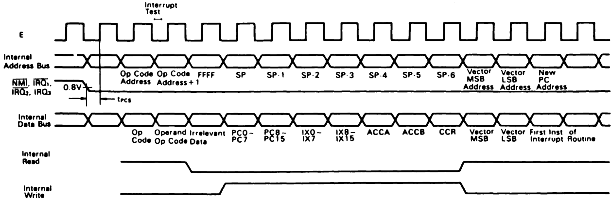
Figure 10 Interrupt Sequence
