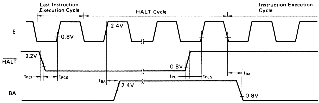
Figure 3 \overline{\text{HALT}} and BA Timing
