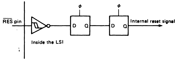
Figure 36 Reset Circuit
