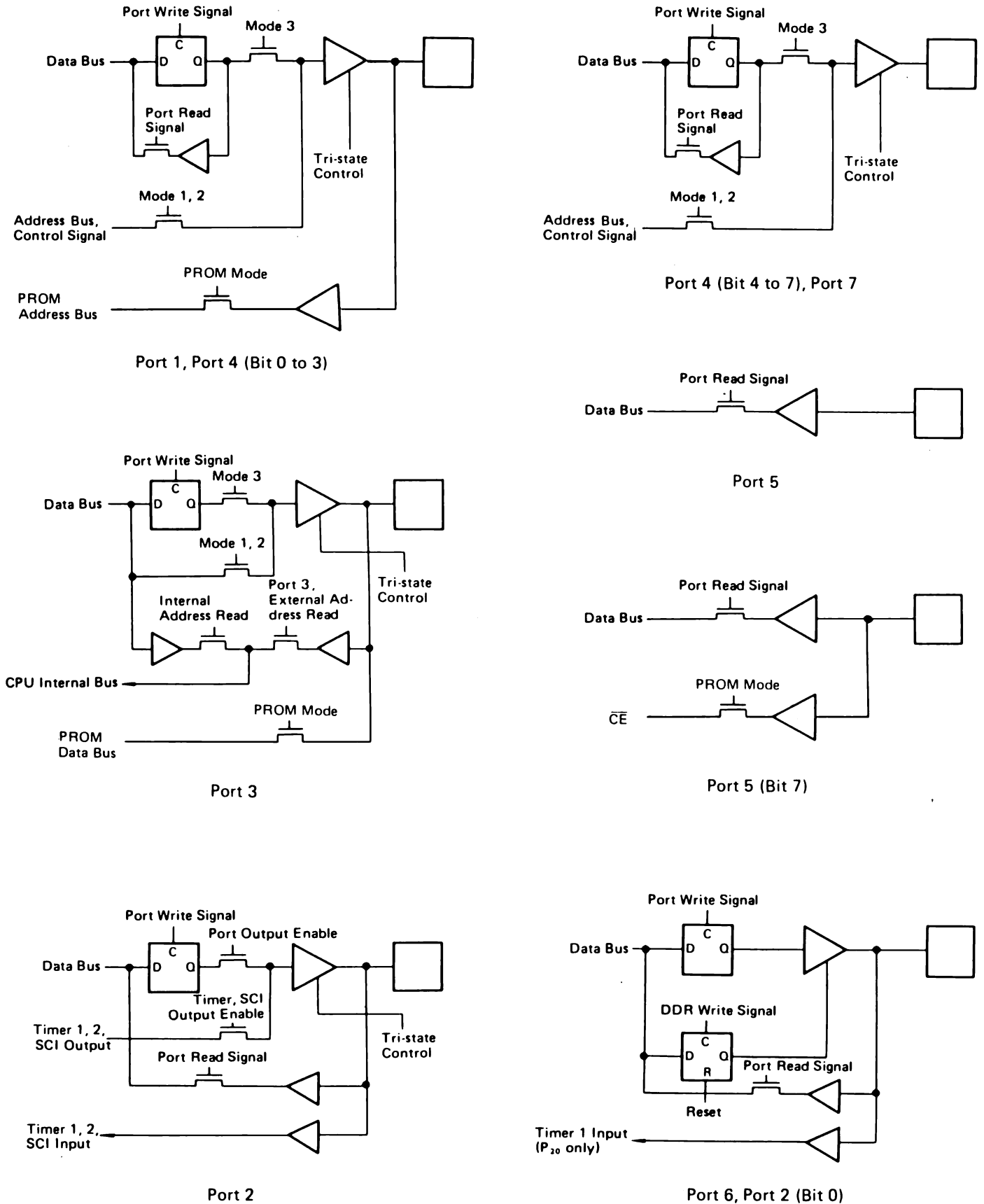
Figure 15 Port Block Diagram
