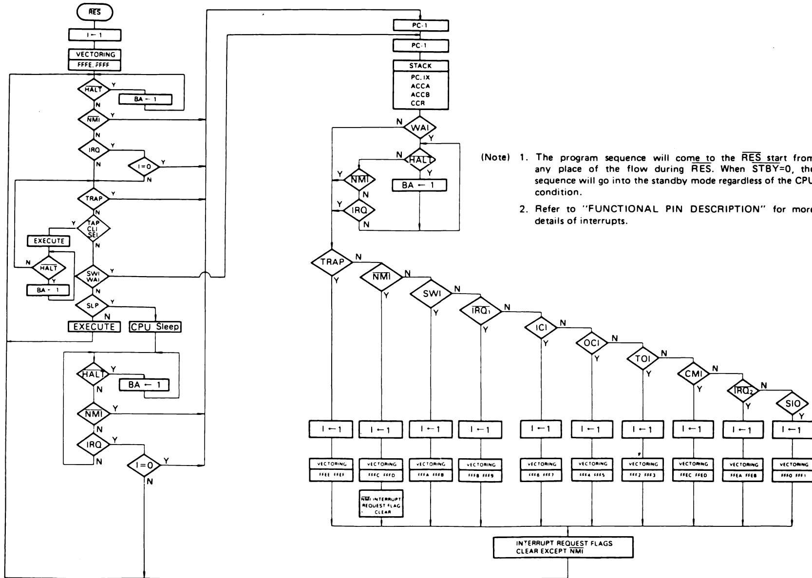
Figure 29 HD63701X0 System Flow Chart
