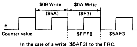
Figure 21 Counter Write Timing
